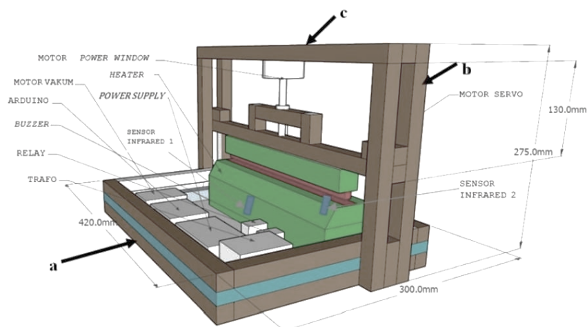
Gambar 2. Design Konstruksi Vacuum Sealer (Afrinda & Myori, 2019)
